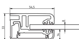
Walk In Easy Comfort Wandanbindung
