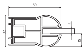
Walk In Easy Comfort Wandanbindung
